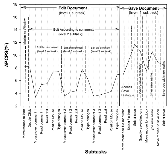
Figure 5: APCPS for subtasks in the document editing task. Solid lines indicate level 1, heavier dashed lines indicate level 2, and lighter dashed lines indicate level 3 boundaries. The x-axis enumerates the observable operators.
